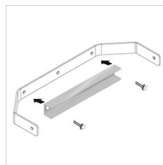
14461104 GUELL 3 strengthening bracket. Suitable for one floodlight single point fixing M10 screw in centre of the bracket.
